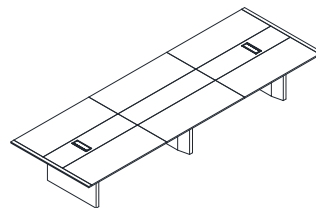
A款会议桌 PJE-MTA-4816 尺寸: 4800W*1600D*760H PJE-MTA-4216 尺寸: 4200W*1600D*760H
